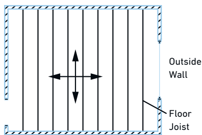
Figure 5: Arrow indicates straight runs parallel to exterior wall to provide warmest water to the coldest area
