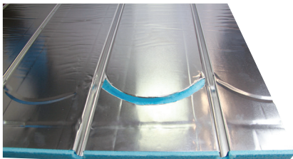
Figure 10: Cut out aluminum to rout PEX in return bends
