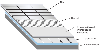
Figure 17: Tile with Xpress Trak on concrete
