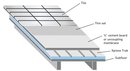
Figure 18: Tile with Xpress Trak on wood subfloor
