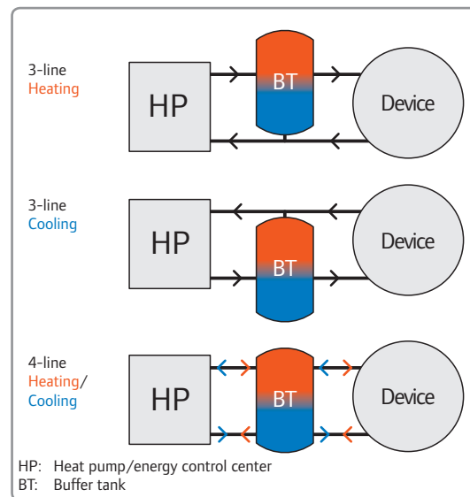
Buffer tanks, connected in parallel
