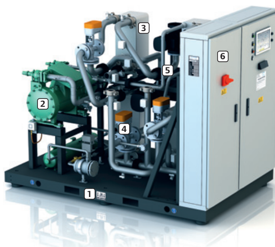
Main components Example: Eco 80 (one module) View without enclosure
