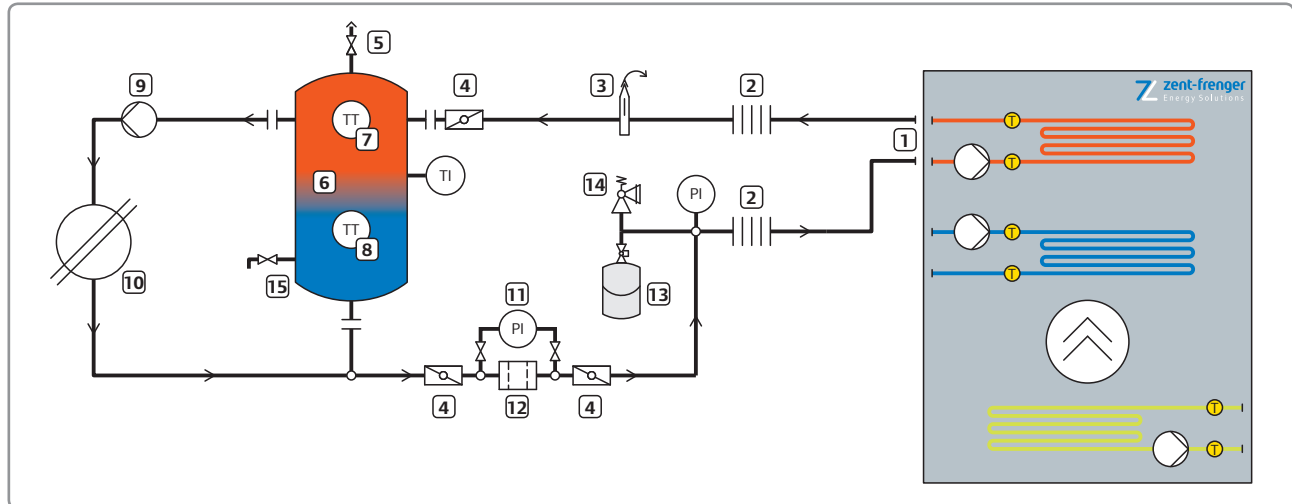
Example hydraulic system
