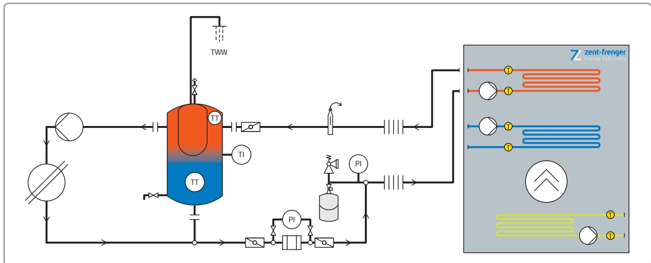
Example hydraulic system Reservoir with calorifier Solution: ideal for high supply temperatures in the heating circuit ( \geq 45^\circ\text{C} )
