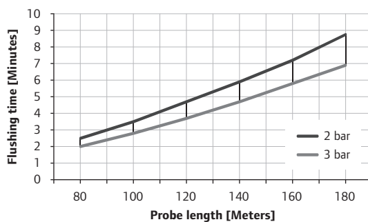
Minimum flushing time for 32 mm probes
