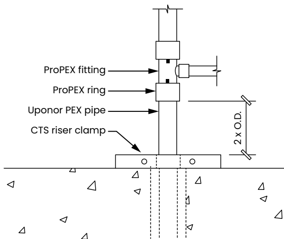
Figure 66: Clamp distance example
