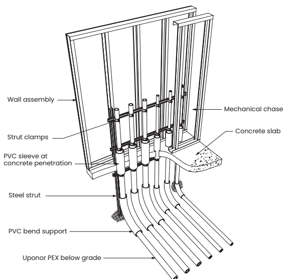
Figure 78: Wet-wall chase transition (below-grade piping)
