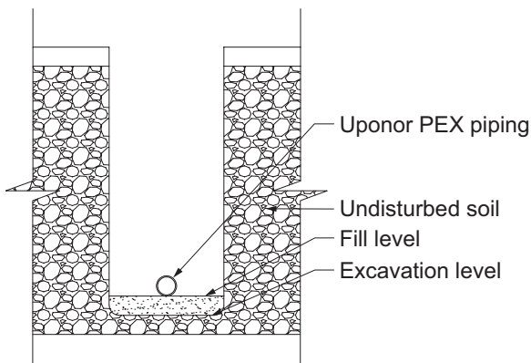
Figure 81: Good soil conditions — If the trench is dug smoothly, install the piping directly on the prepared bottom. The bottom must be flat with no hollows, lumps or rocks.
