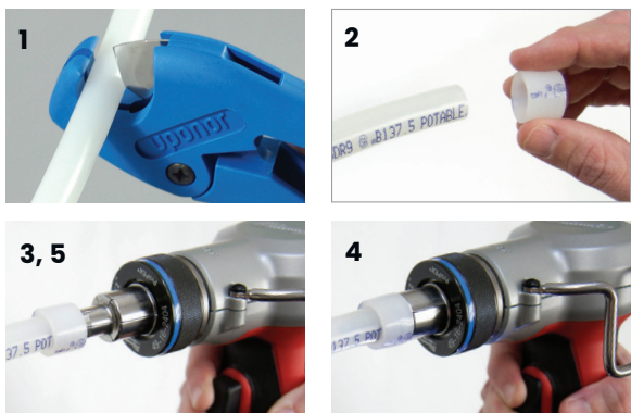
Figure 4: Expansion with Milwaukee M12, M12 FUEL, M18, and M18 FUEL 2" ProPEX expansion tools
