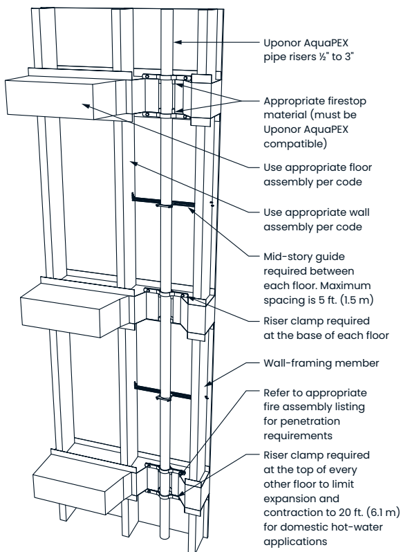
Figure 69: Domestic hot-water riser detail
