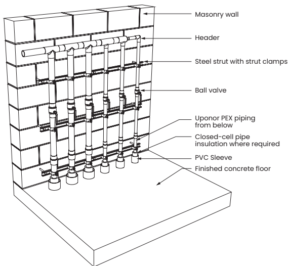
Figure 77: Mechanical room transition (below-grade piping)
