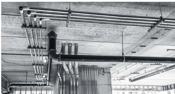
Figure 55: Supporting PEX with PEX-a Pipe Support
