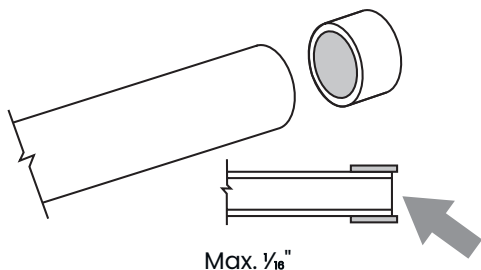
Figure 32: Slide the expanded ring over the end of the piping
