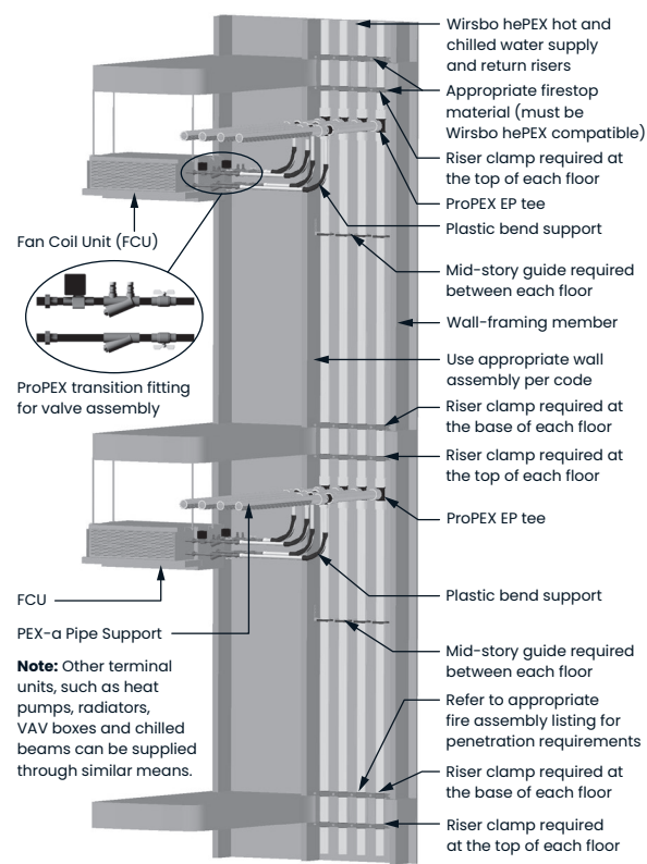
Figure 68: Hydronic piping riser detail
