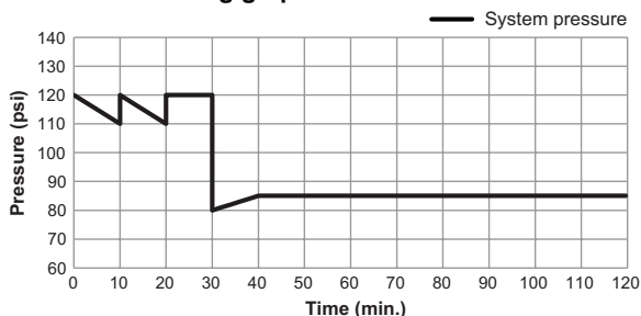
Figure 83: Pressure testing graph
