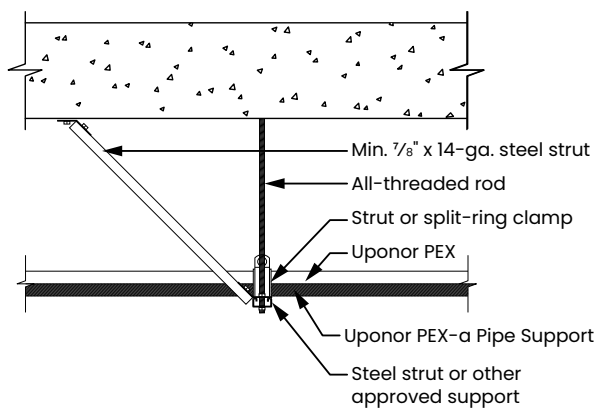
Figure 56: Fixed point
