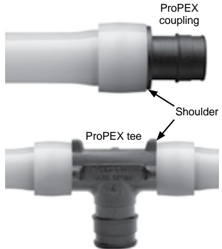
Figure 3-15: Fitting shoulders
