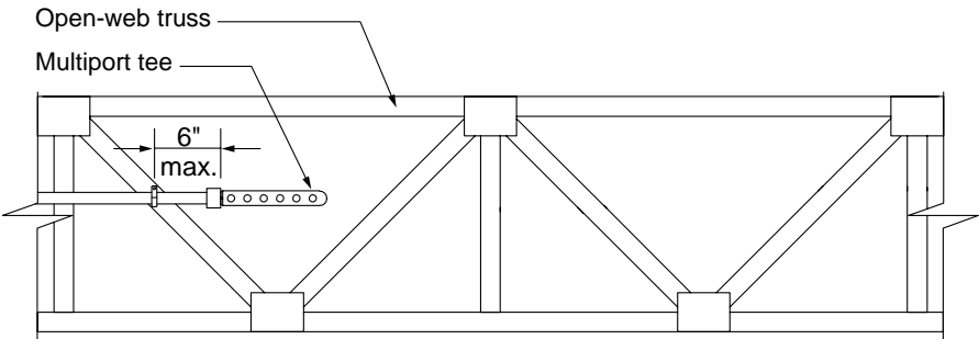
Figure 5-12: Supporting multiport tees on open-web wood trusses
