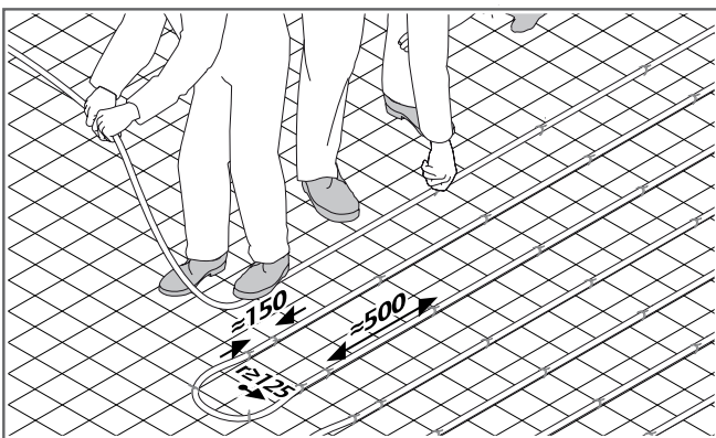
Heating pipes fixated to reinforcement mesh with Uponor Multi cable ties PA.
